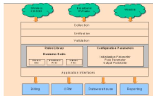
i-Mediator Architecture
